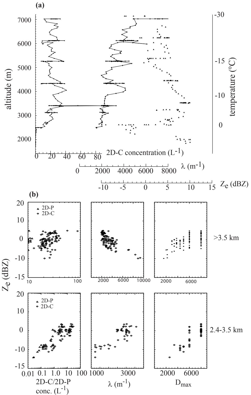
Fig. 7. (a) Vertical profiles of particle concentrations, \lambda , and Z_e during the staircase descent of October 31, 1992. (b) Scatter plots of Z_e versus particle concentrations, \lambda , and maximum bin size where particles were detected.
