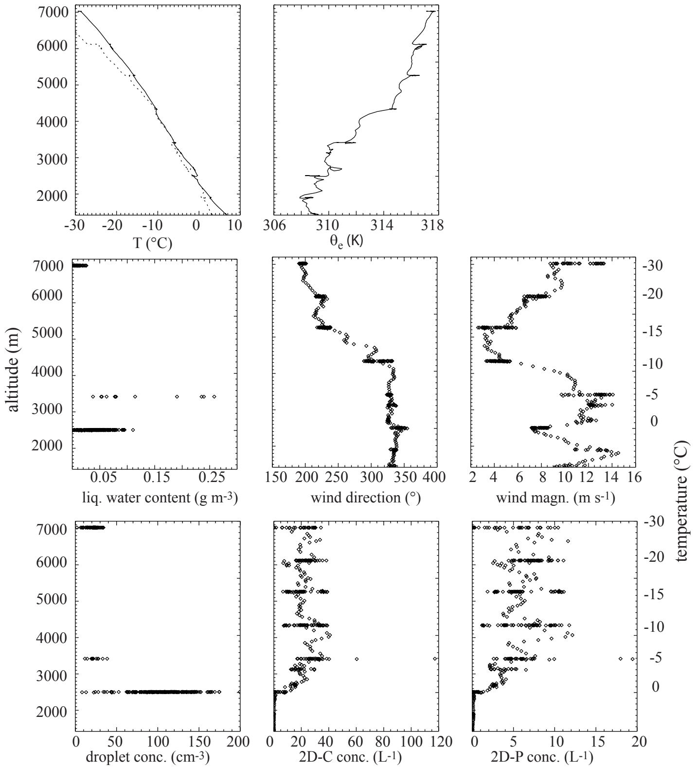
Fig. 3. Vertical profiles of different parameters during the staircase descent on October 31, 1992. The dashed line in the first panel is dew point temperature.
