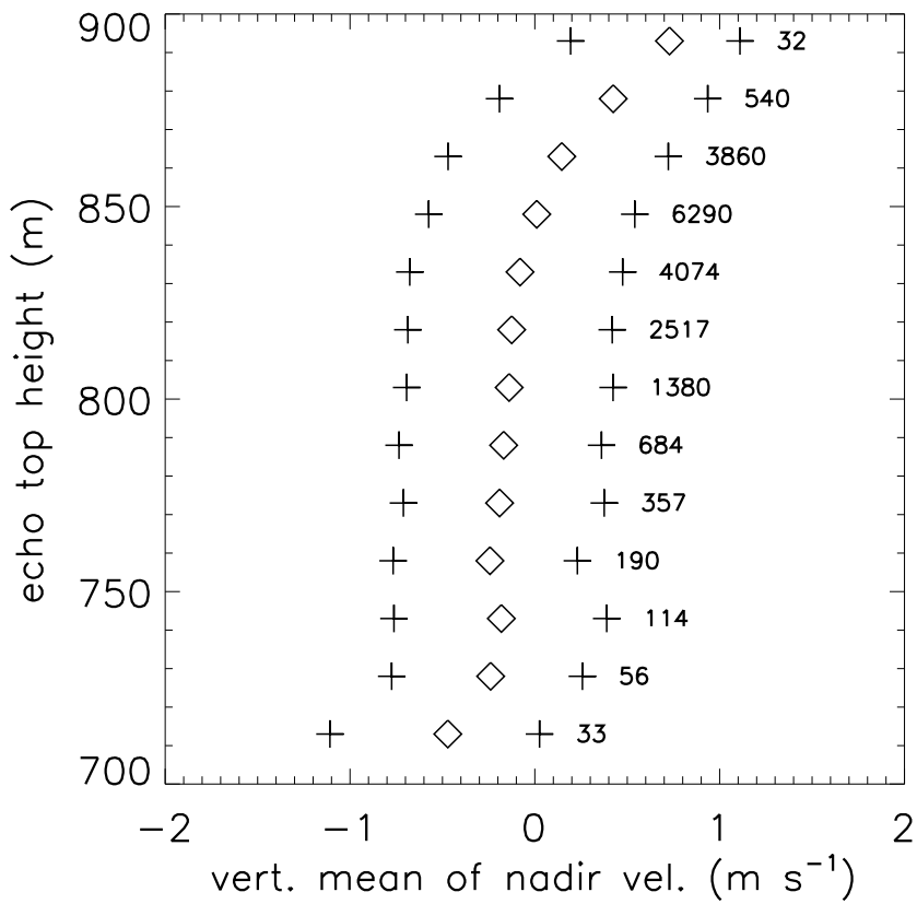
rf05 1030-1058 echotop vs. vertical mean of nadir velocity
