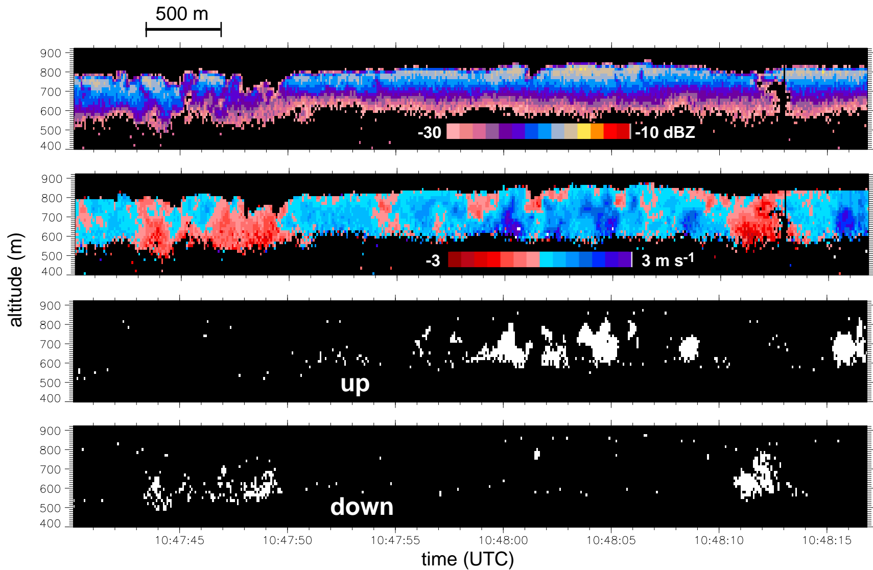
rf05 circ_1030; 12684:13134; 0:35. Highlighted velocities >+1\text{ m s}^{-1} and <-1\text{ m s}^{-1}
