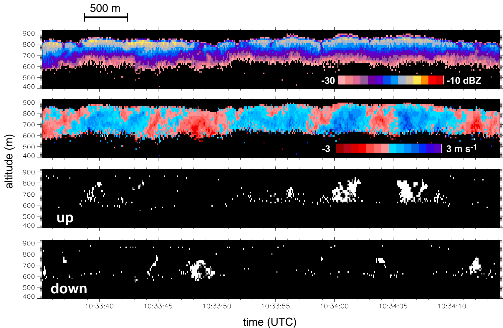
rf05 circ_1030; 2365:2815 0:35. Highlighted velocities >+1\text{ m s}^{-1} and <-1\text{ m s}^{-1}
