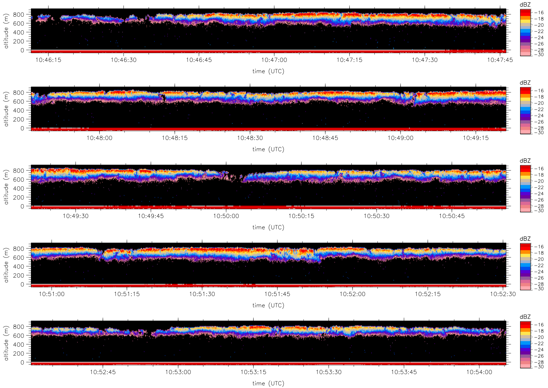
rf05_1030-1058 10:46:11 to 10:54:05 Second level look at WCR nadir beam reflectivity. Vert. range = 0:66
