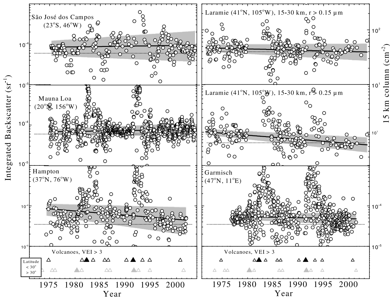
Figure 8. Same as Figure 7, except the data points are the measurements with the volcanic effect estimated from the model subtracted. The residuals for Laramie in 1980, following Mt. St. Helens, are off scale since Mt. St. Helens was not included in the model for Laramie.
