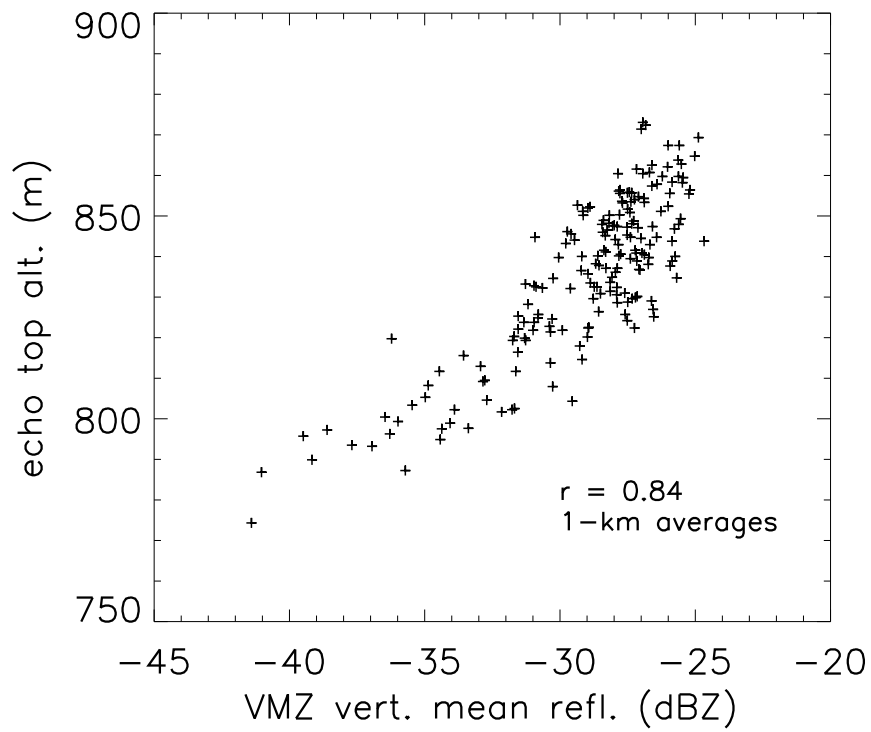
Echo top height vs. VMZ. rf05_1030-1058
