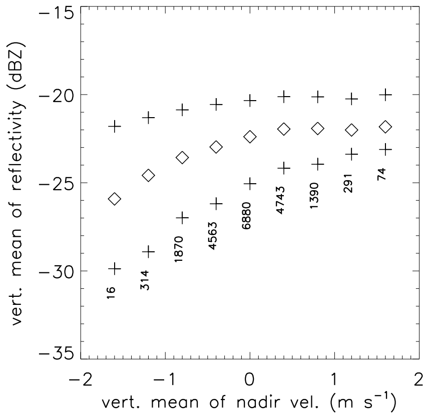
rf05 1030–1058, vert. mean reflectivity vs vnadir velocity
