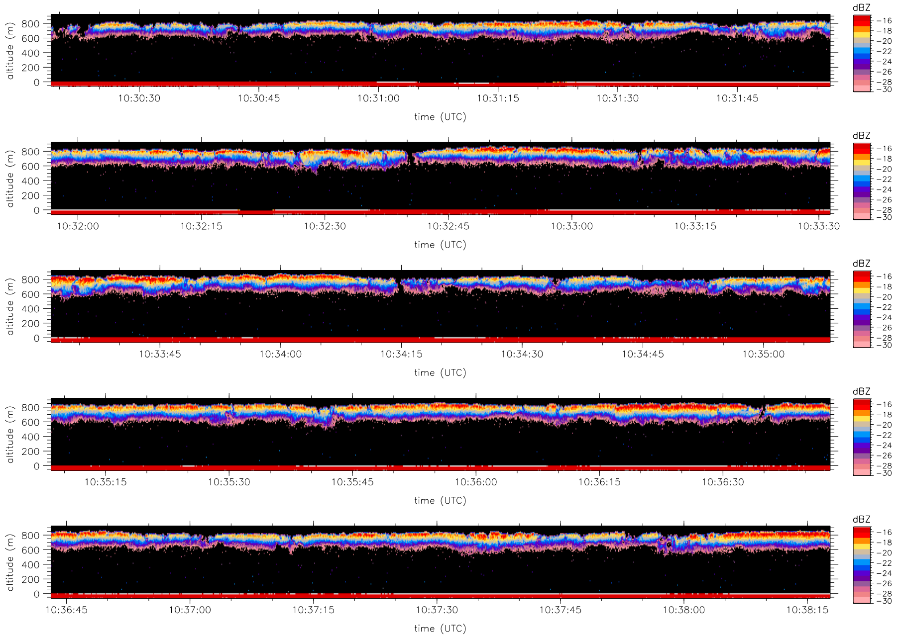
rf05_1030-1058 10:30:18 to 10:38:17 Second level look at WCR nadir beam reflectivity. Vert. range = 0:66
